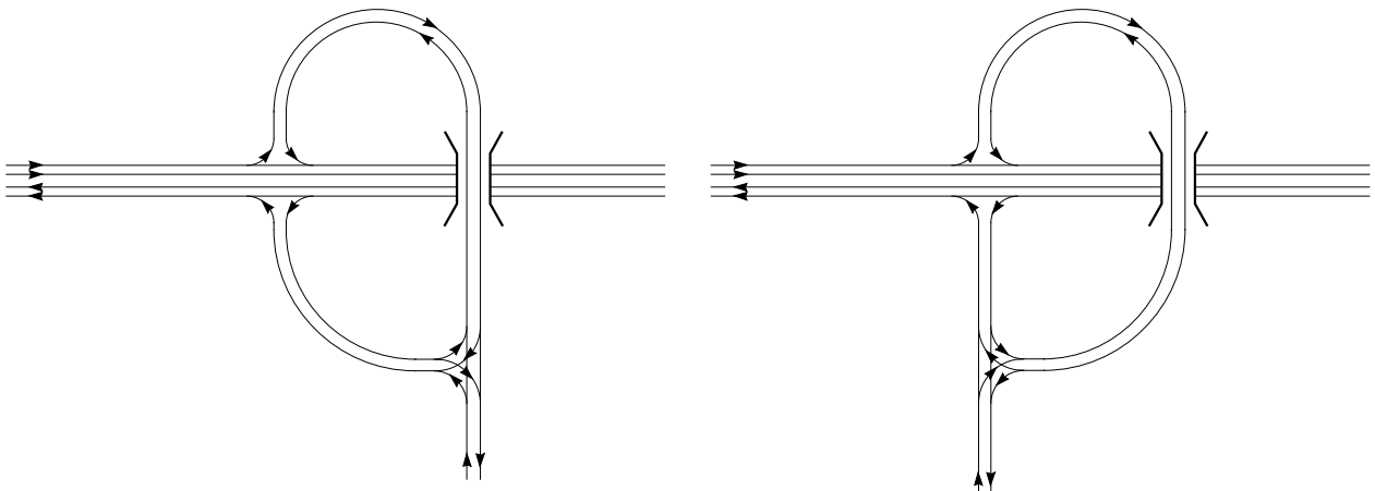
Figure 7/7 Schematic Examples of 3 Arm Compact Grade Separation on Dual Carriageways
